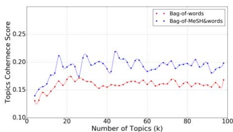
Figure 2- Comparison of mean TC-W2V topic coherence scores for different numbers of topics k , generated from the specialized corpus
