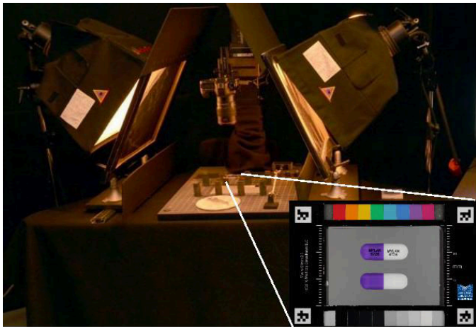
Fig. 1. Reference image macro photography rig. Inset shows the macro calibration card placed on top of floating stage and the imaged pills.
