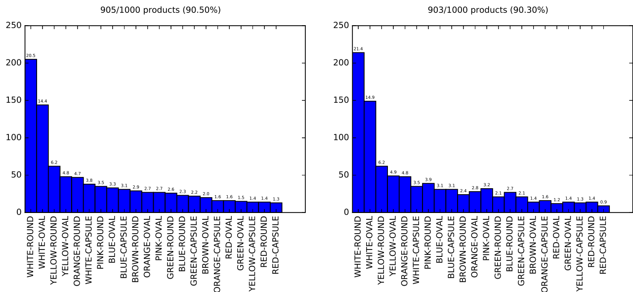
Fig. 3. Distribution of pills based on their key visual properties, shape and color. (left) training data and (right) segregated testing. The segregated testing dataset is comprised of reference and consumer quality images from products that were not part of the training set.
