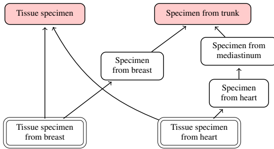
Figure 5: Non-lattice pair from the Specimen hierarchy.
